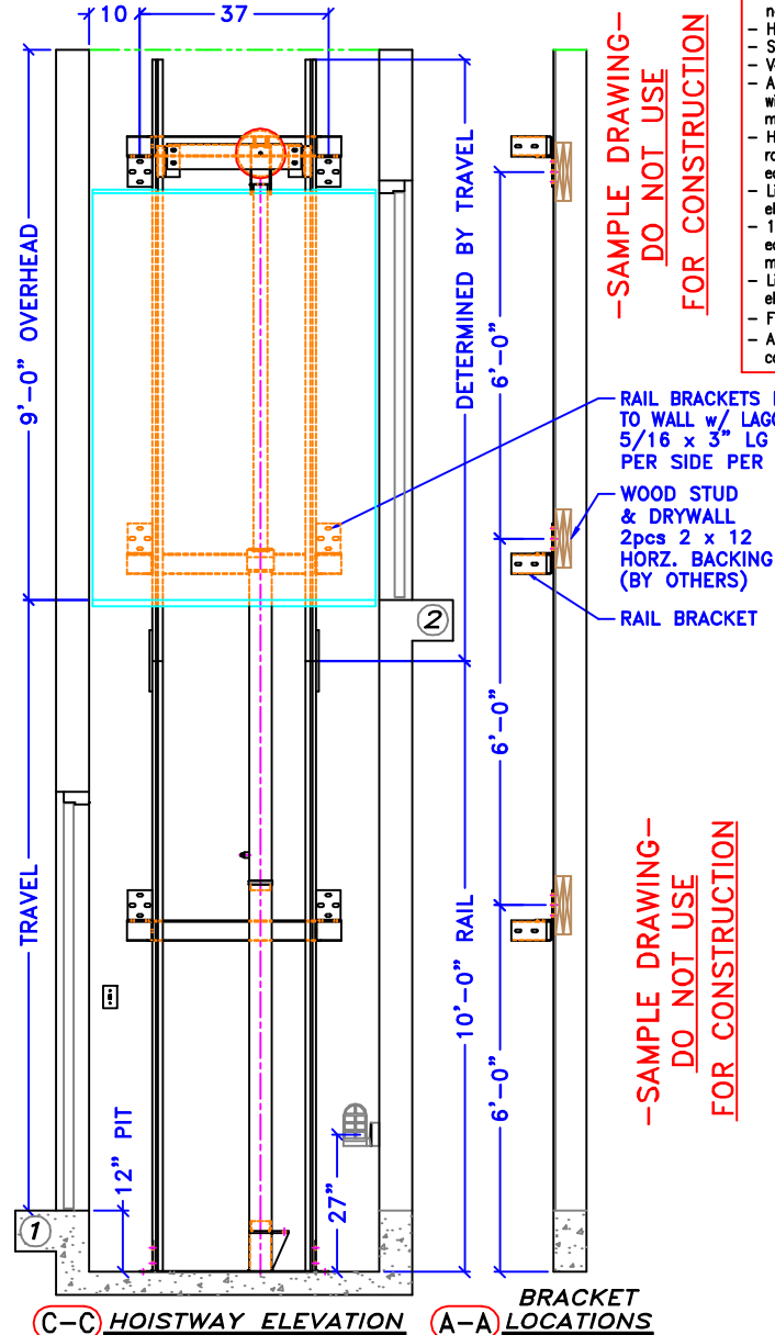
C-C HOISTWAY ELEVATION A-A BRACKET LOCATIONS
